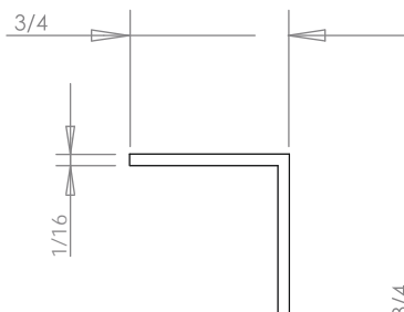
Section view
