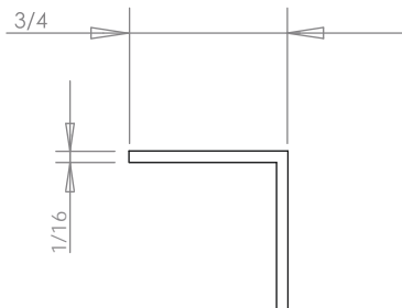
Section view
