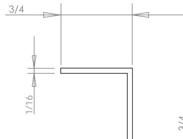
Section view
